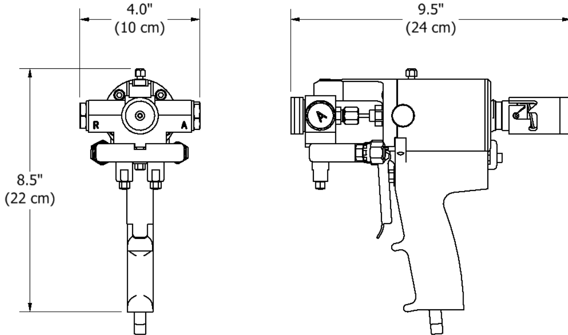
Figure 1: PX-7 Dimensions
