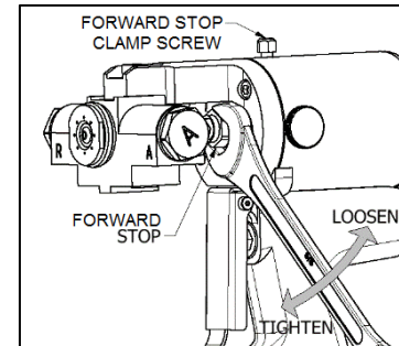
Figure 12: Valving Rod Adjustment
