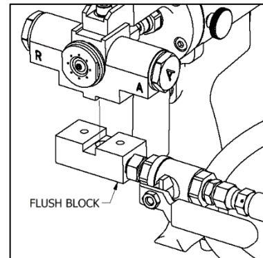
Figure 15: Flush Block Installation
